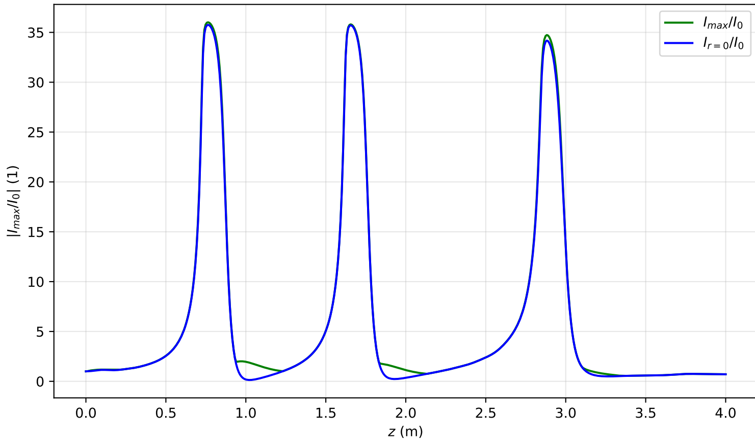
I_{max}(x=0, y=0, z)/I_0 , Pin=3.0Pcr, noisy input, artificial time
